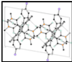
Fig. 2. A packing diagram of the title compound, viewed down the b axis. Hydrogen bonds are shown as dashed lines.
